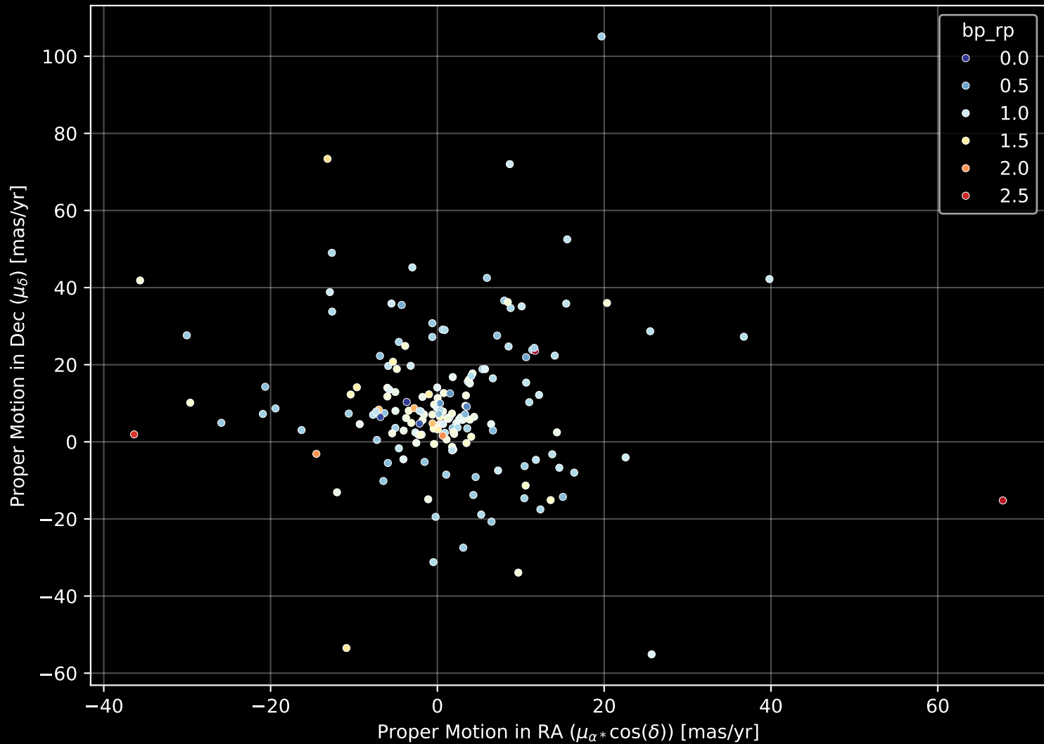
APOGEE DR17 Field: [265-28-O_TESS] Proper Motion Diagram (n= 179)
