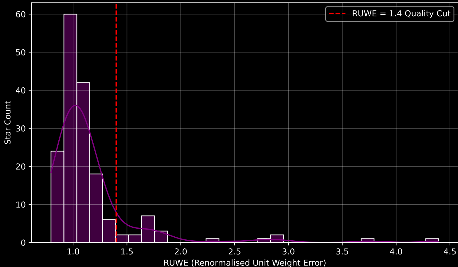
GAPOGEE DR17 Field [265-28-O_TESS] RUWE Distribution (n= 170)
