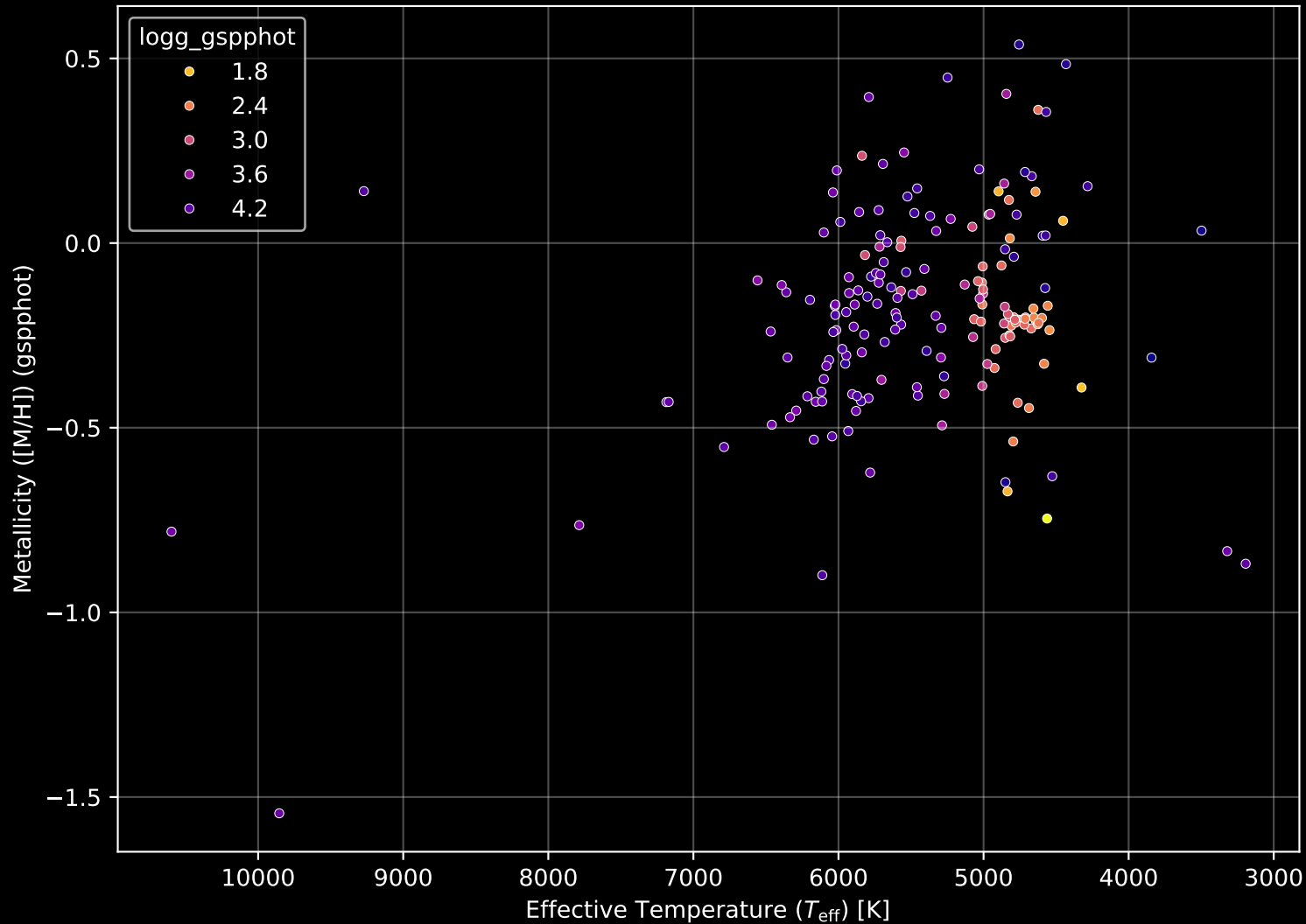
APOGEE DR17 Field: [265-28-O_TESS] Stellar Population Parameters (n= 179)
