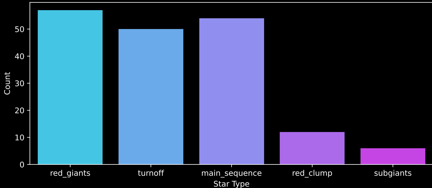
APOGEE DR17 Field: [265-28-O_TESS] Count plot of Star Type
