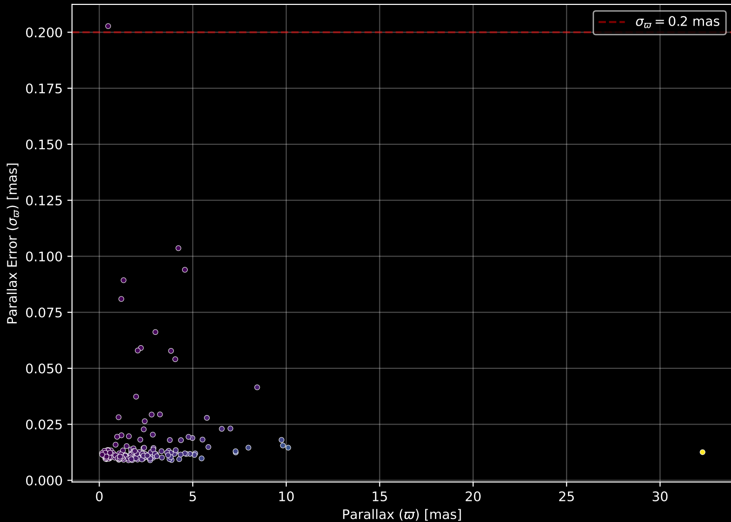
APOGEE DR17 Field: [265-28-O_TESS] Parallax Quality (n= 179)
