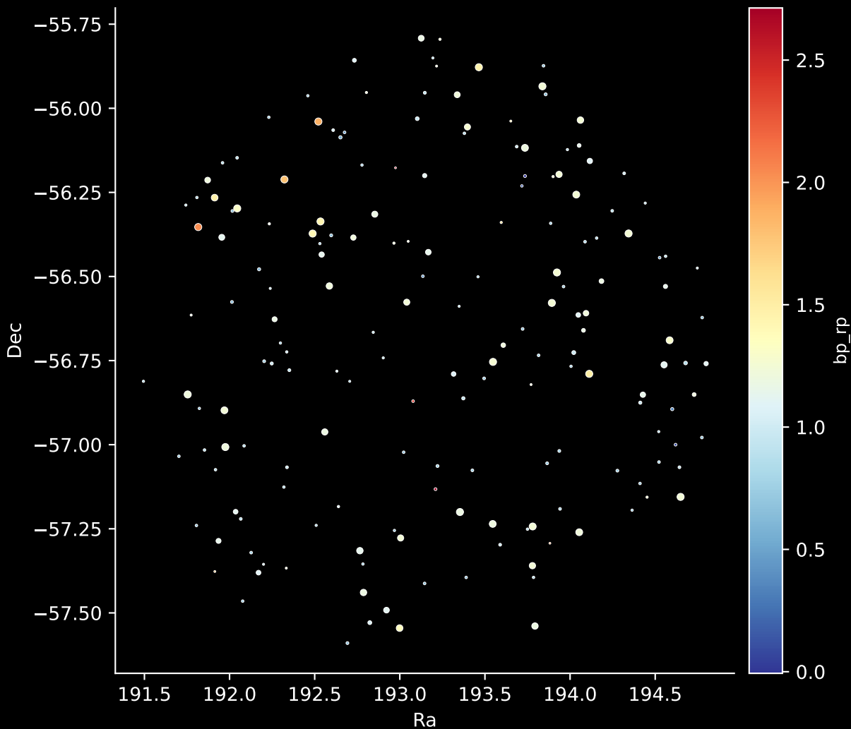
APOGEE DR17 Field: [265-28-O_TESS] Stars: 179
