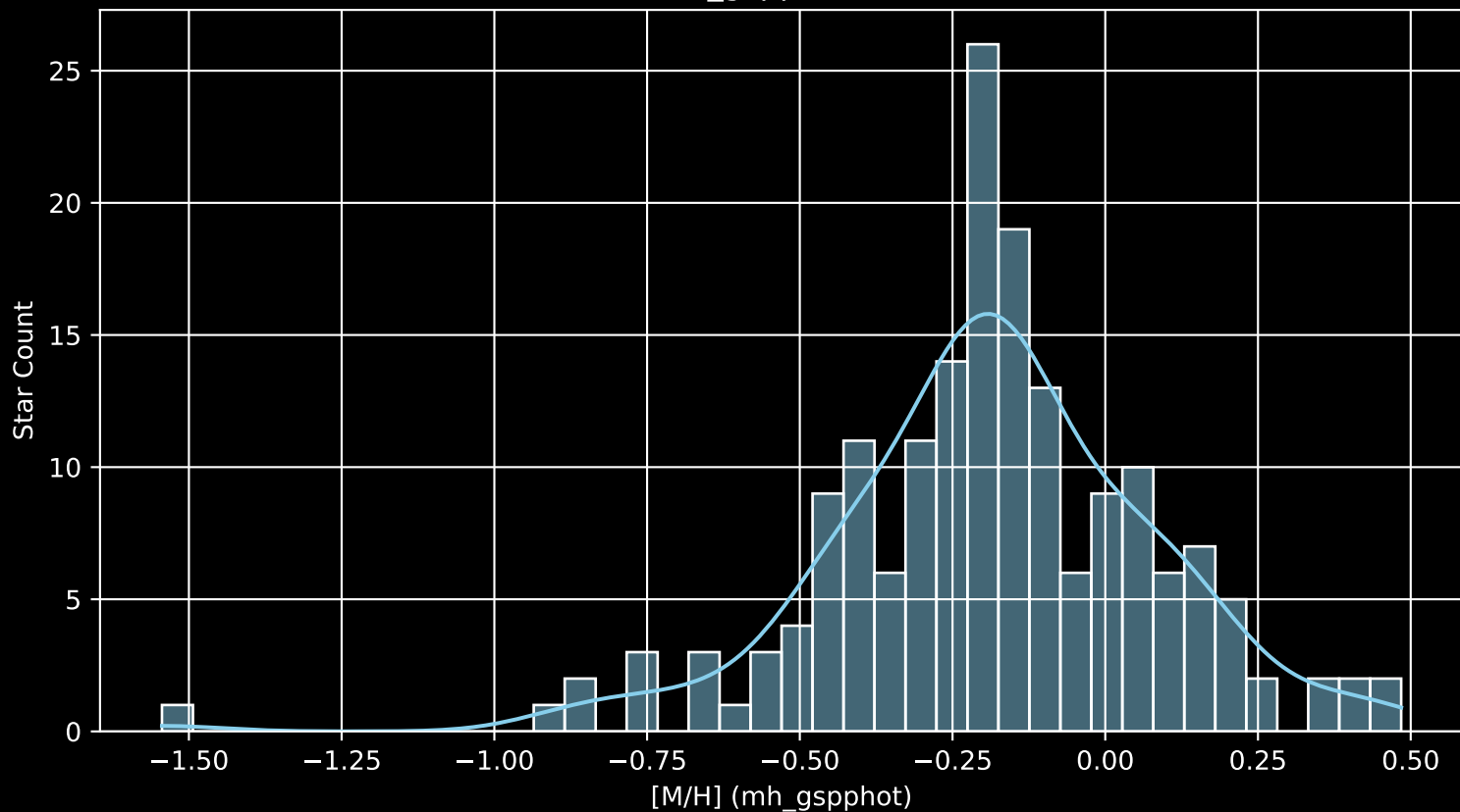
APOGEE DR17 Field: [265-28-O_TESS [M/H] (mh_gspphot) (n= 178)
